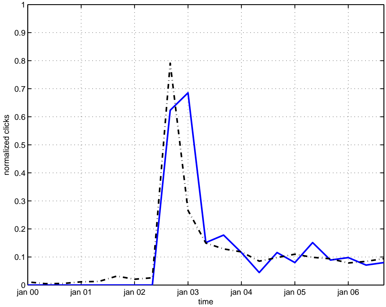
a(8) algebra
