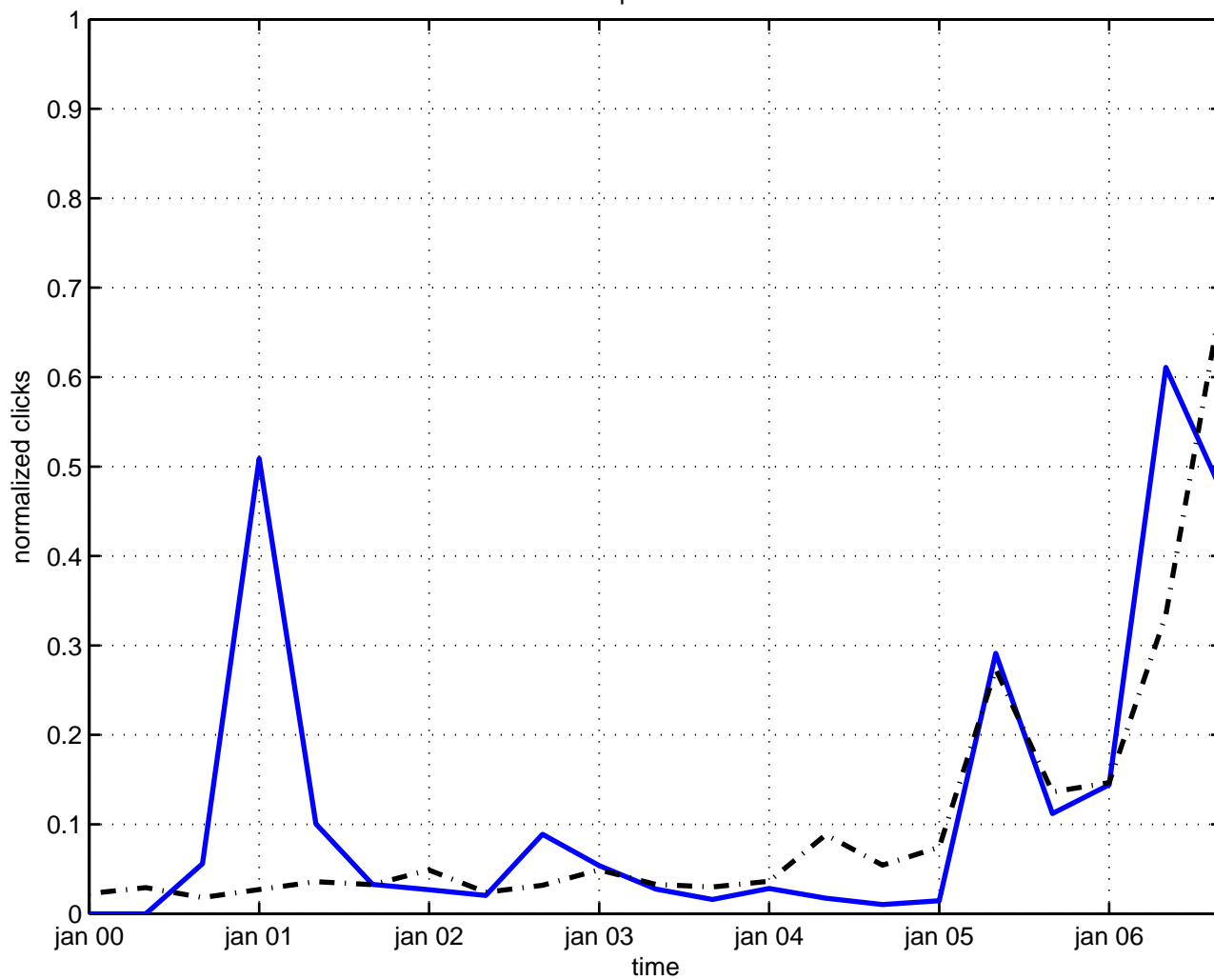
8 p-brane
