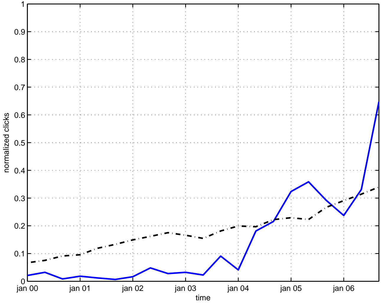
7 p-brane
