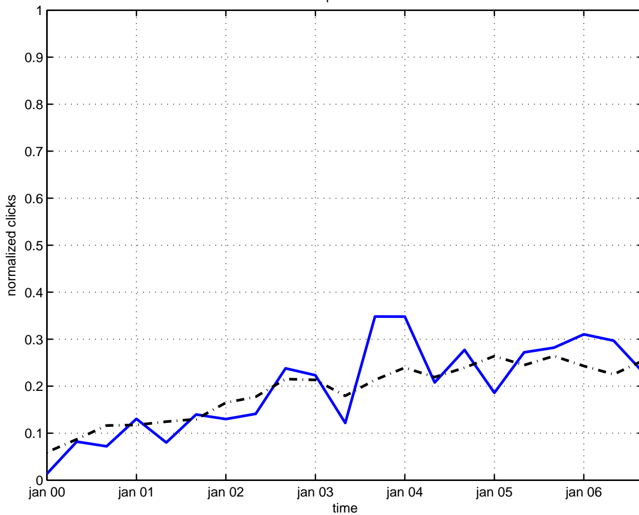
6 p-brane
