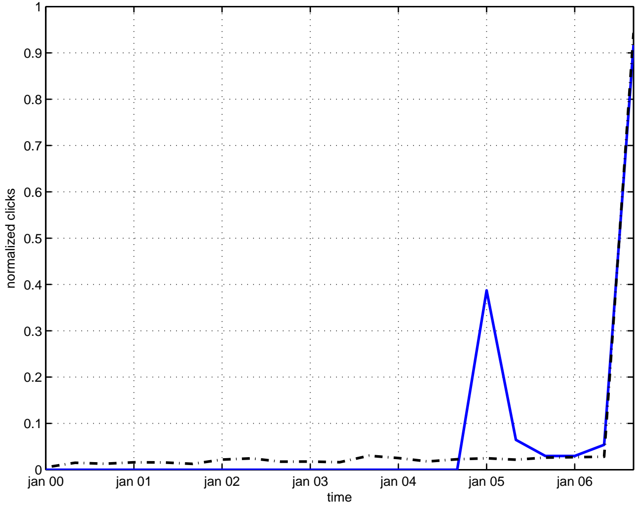
6 n-point function
