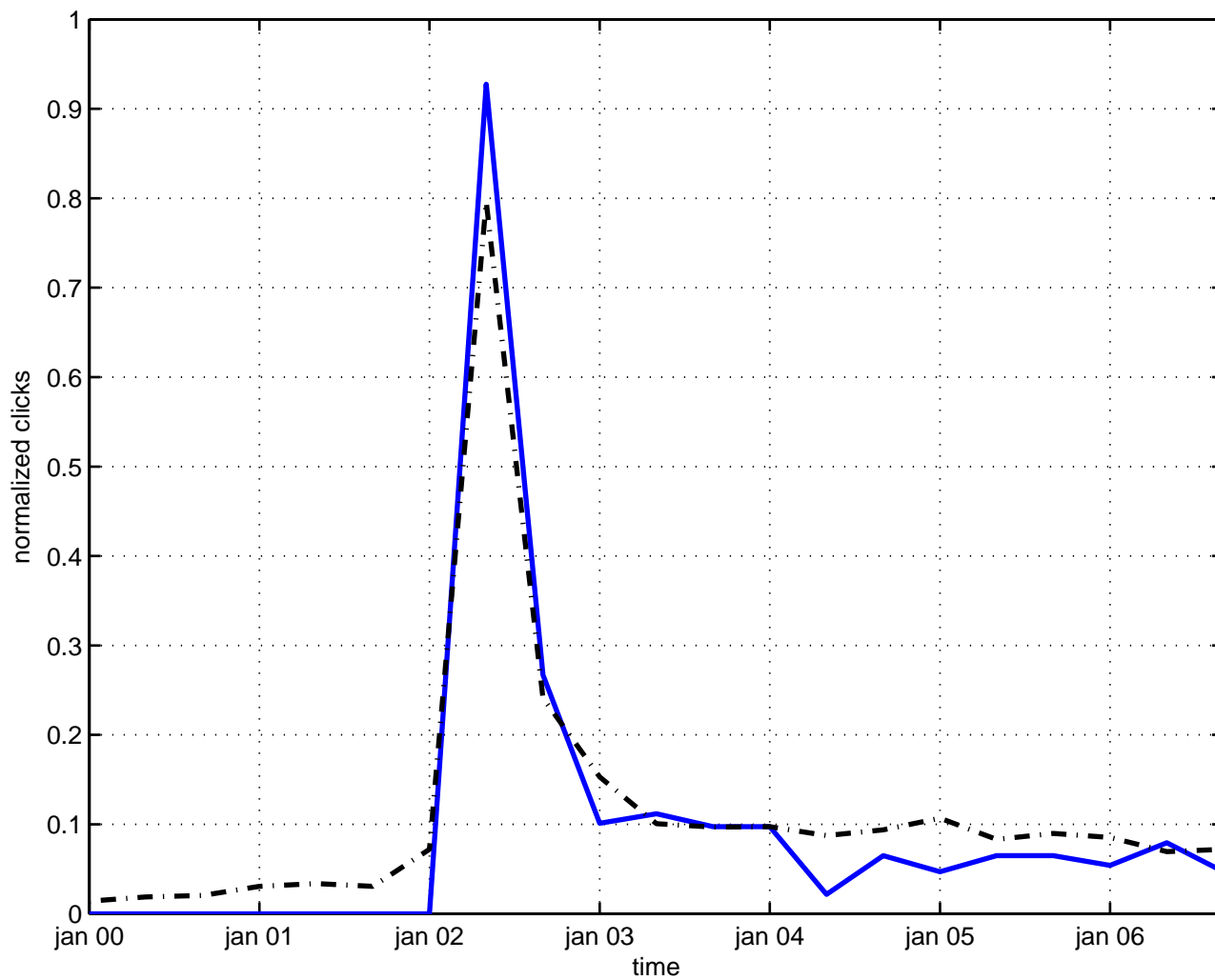
6 d-brane
