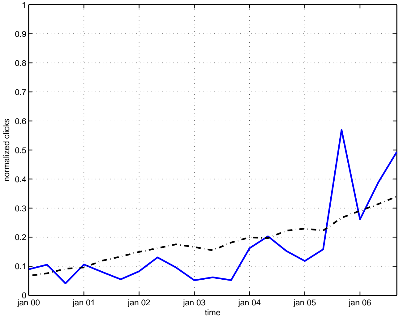
4 p-brane
