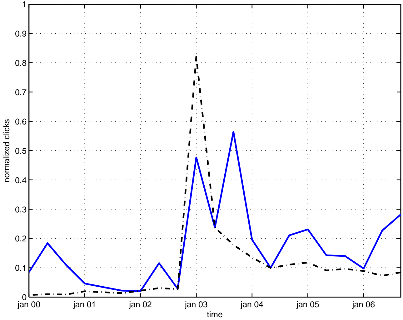
4 differential forms
