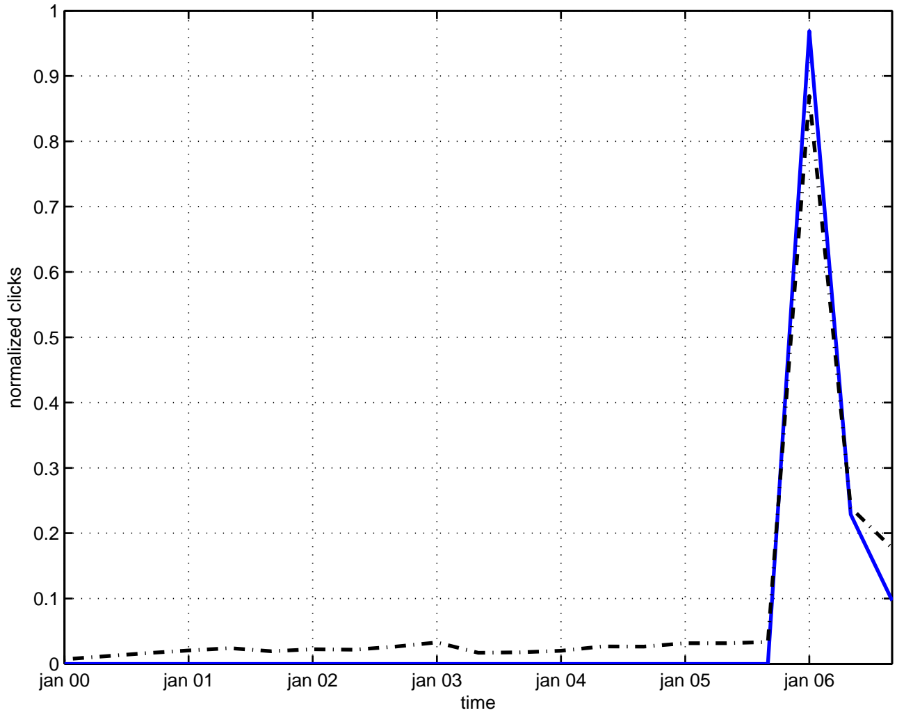
3 matrix model
