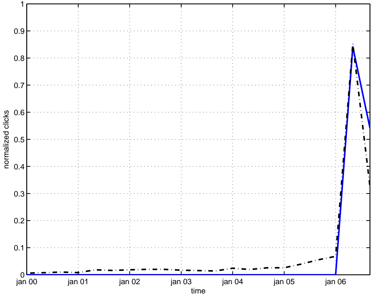
3 fermion number
