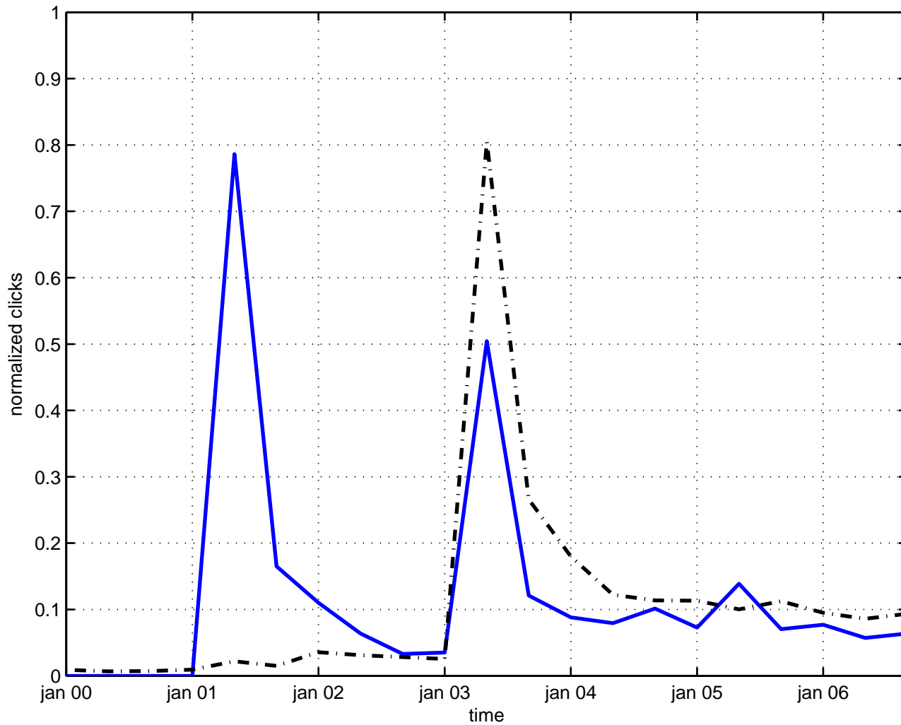
3 d-brane
