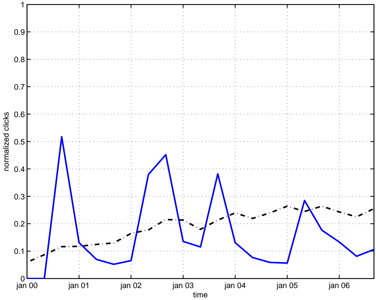
25 p-brane
