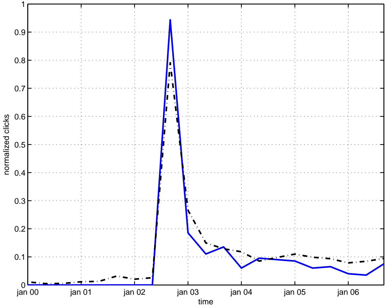
23 p-brane
