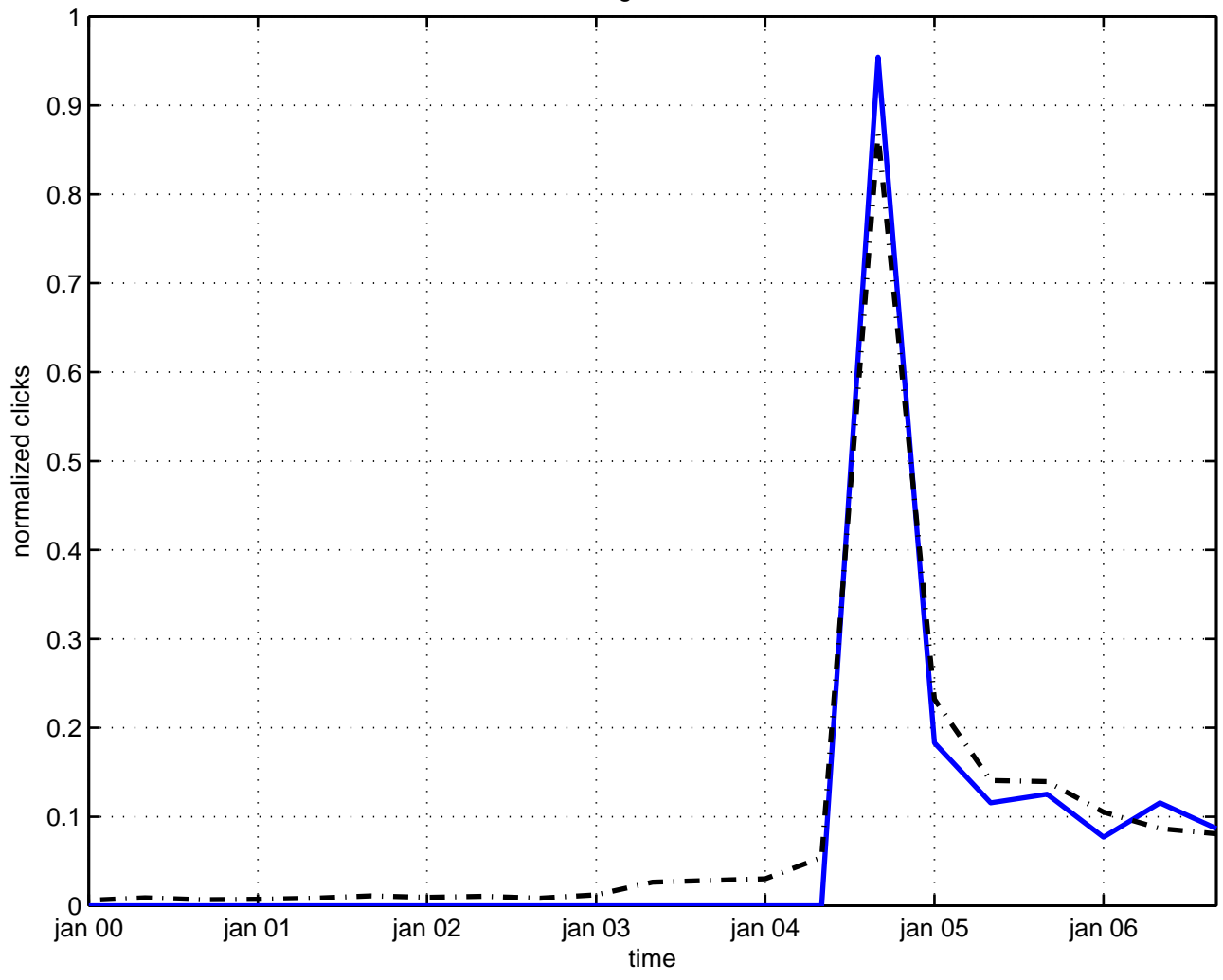
2 graviton
