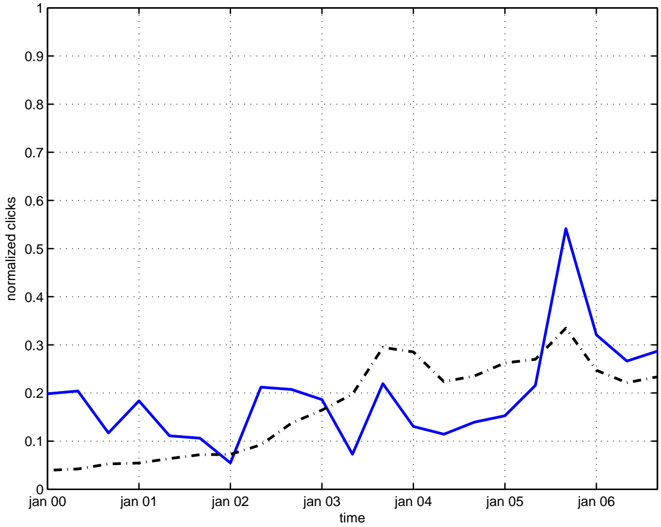
0 p-brane
