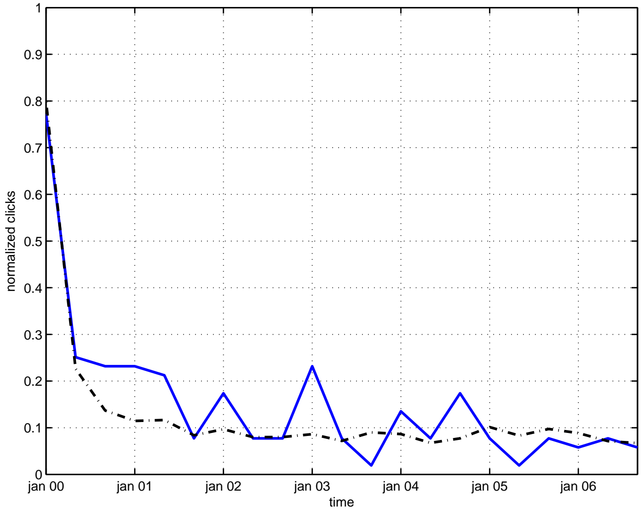
0(3) symmetry
