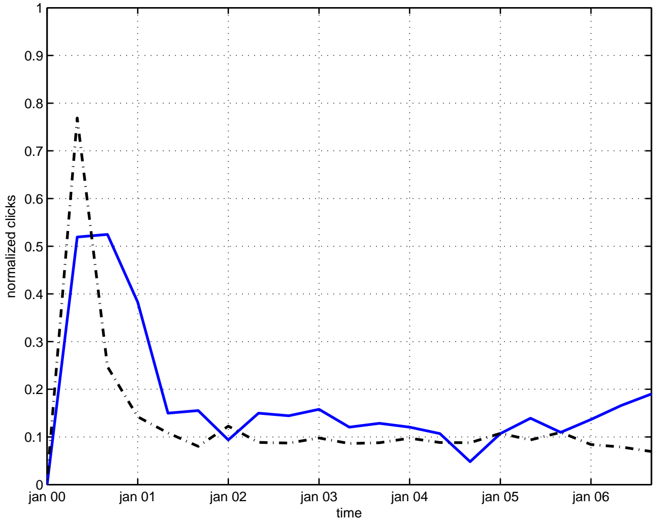
(higgs particle radion) coupling
