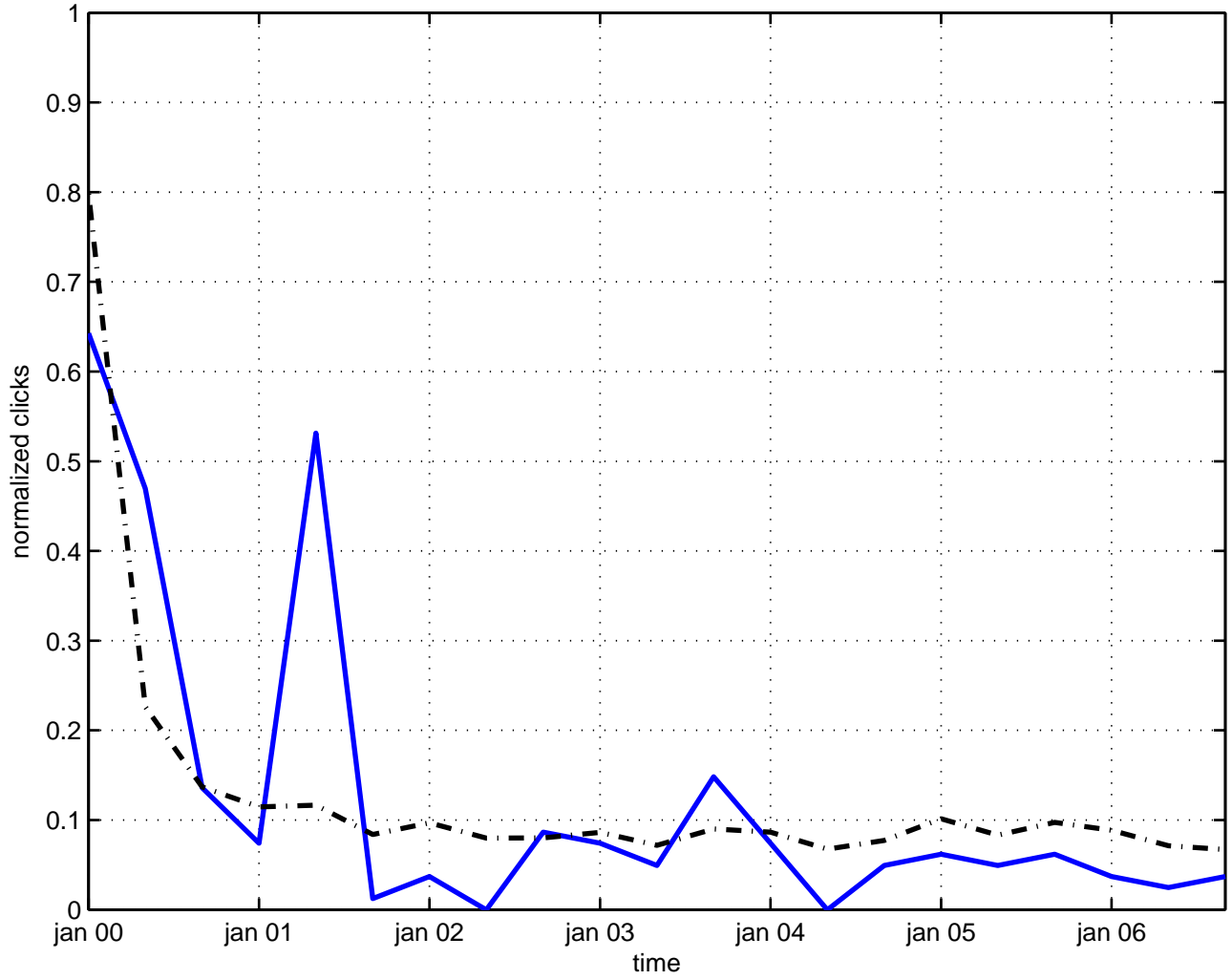
(3fermion) bound state
