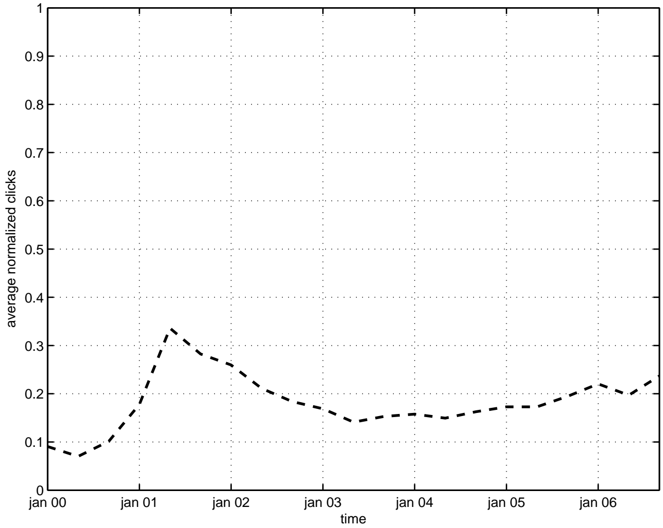
cluster 20 (130 topics)
