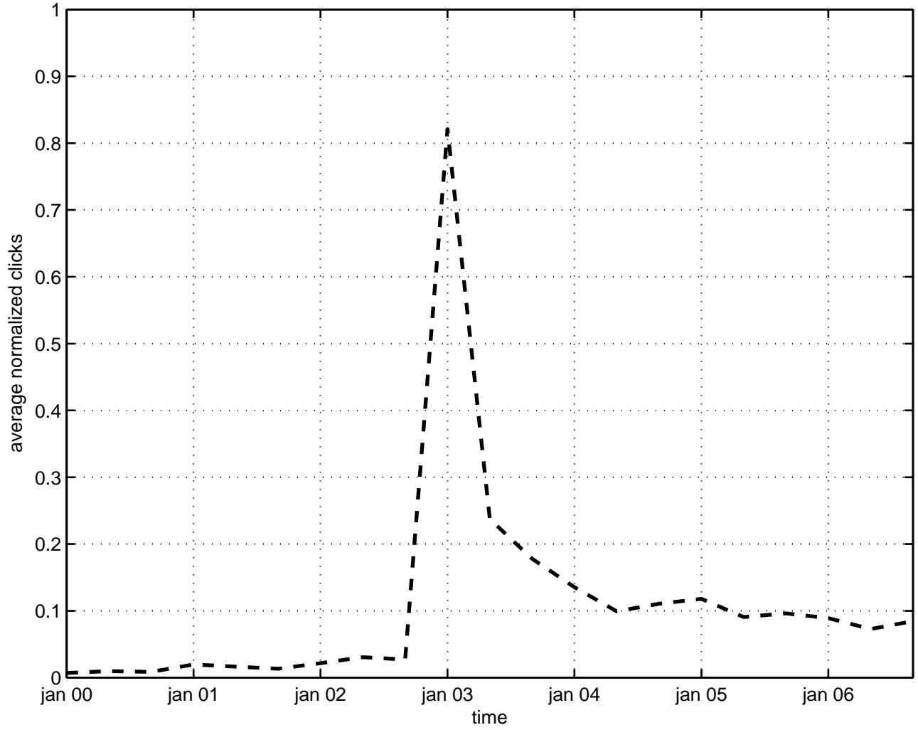
cluster 9 (318 topics)
