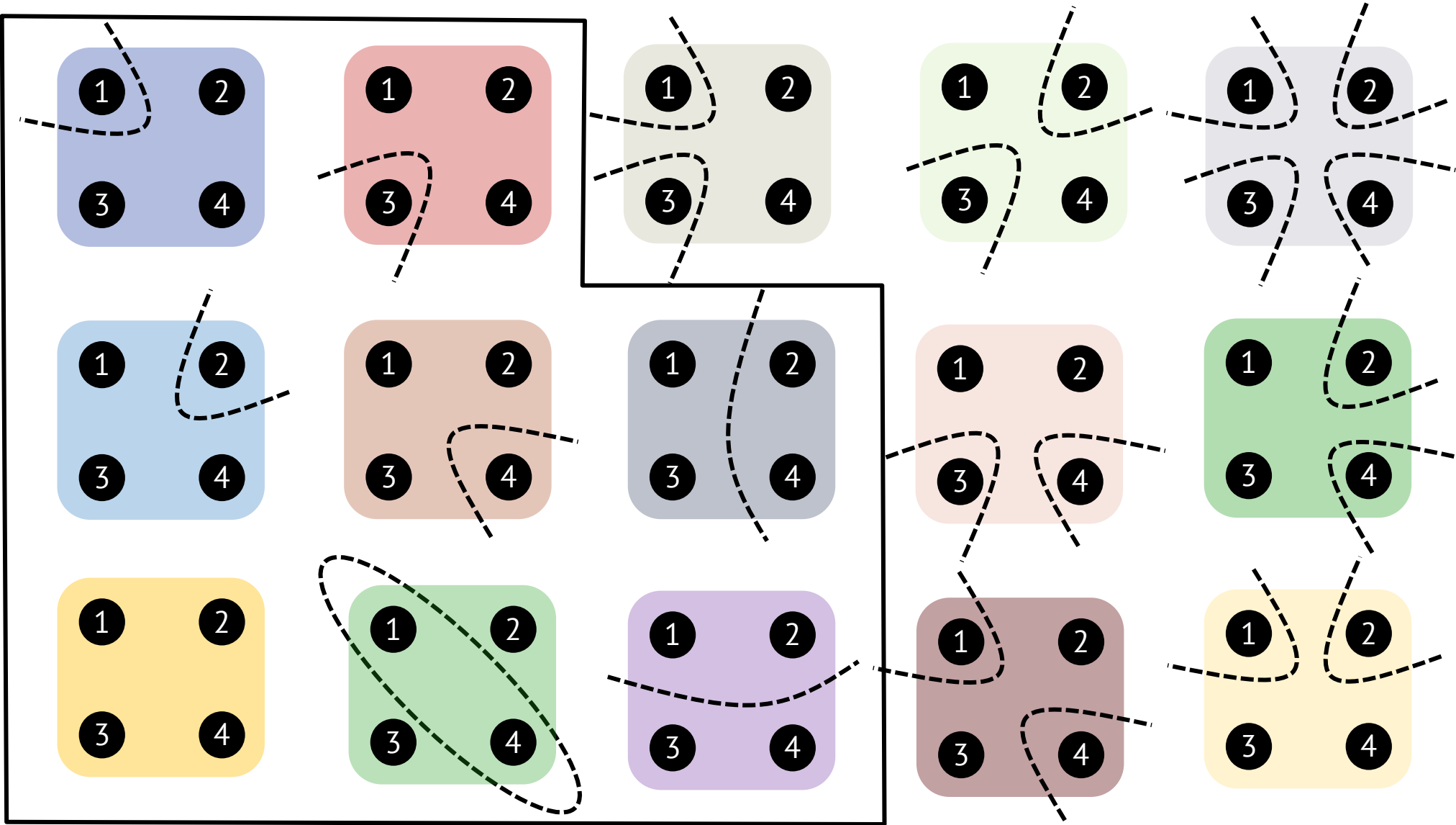
Seven when restricting to two clusters.
