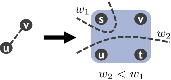
Reduction from max cut
