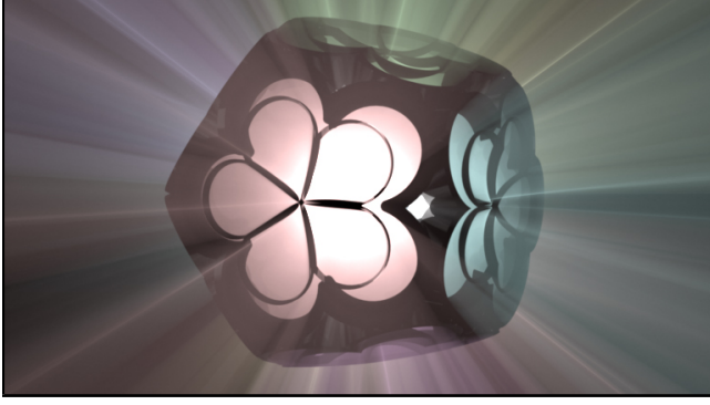
Figure 9: It is possible to extend the path space specular integration framework to volumes, for instance to render caustics from refractive objects, such as this dodecahedron-shaped luminaire with tinted glass inlays.
