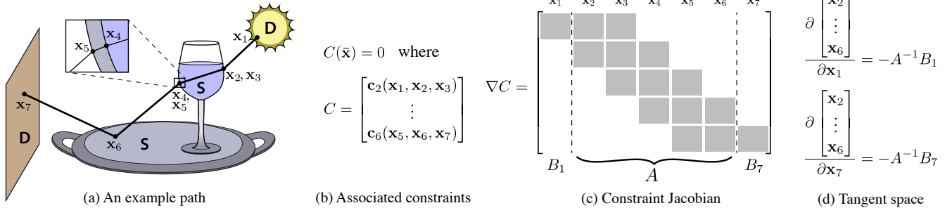
Figure 2: The linear system used to compute the tangent space to the specular manifold, also known as the derivative of a specular chain with respect to its endpoints.
