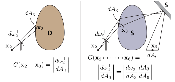
Figure 3: The geometry factor (left) and the generalized geometry factor (right) are both derivatives of projected solid angle at one end with respect to area at the far end.
