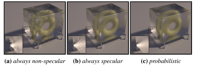
Figure 8: Consistently classifying glossy materials as non-specular or specular produces unsatisfactory results. Instead, our method makes this decision randomly whenever encountering a rough object (modeled after a scene by Cline et al.)
