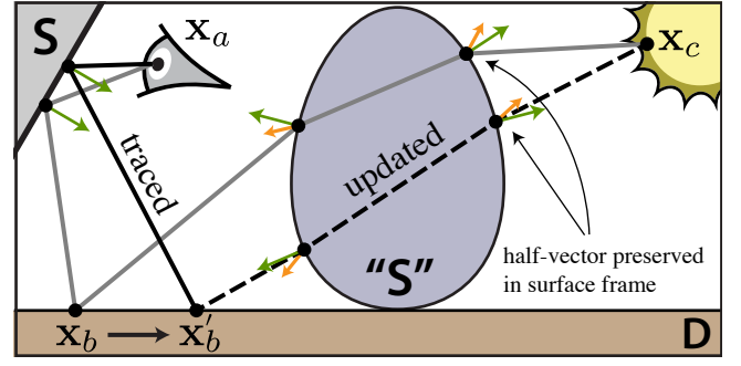
Figure 7: Perturbation of path with near-specular surface interactions: instead of requiring that the half-vectors agree with the surface normals, their direction is preserved in the surface frame.
