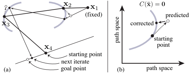
Figure 4: One iteration of updating a path using the specular manifold. (a) The path vertices are modified according to a local linear model, which (b) corresponds to a step along the tangent plane to the manifold, then (a) a nearby valid specular path is found, which (b) corresponds to projecting back onto the manifold.
