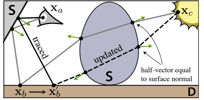
Figure 6: Manifold perturbation example: a slightly perturbed outgoing direction at \mathbf{x}_a is propagated until encountering the non-specular vertex \mathbf{x}'_b . Previously, it was not clear how to “connect” \mathbf{x}'_b to \mathbf{x}_c through multiple specular interactions. Our method can find this connection given knowledge about the previous path.
