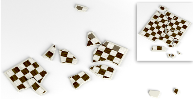
Figure 5: Bigger “cracks” with fracture impulses: Our quasistatic fracture impulses produce more explosive fractures, thereby producing louder and more characteristic “crack” sounds. In contrast, simulations without fracture impulses applied (see inset) lack fracture-released kinetic energy. This ceramic chessboard (38cm × 38cm) was dropped from one meter high onto the ground.
