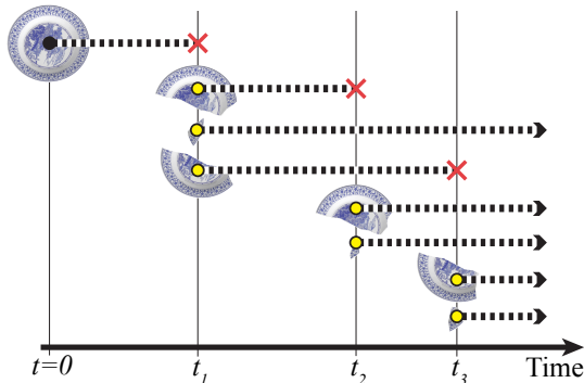
Figure 3: Time-varying rigid-body sound models are used to approximate fracture sounds. Discrete fracture events result in spectral discontinuities due to modal sound model destruction (X) and creation (●). Fracture impulses excite created sound models.
