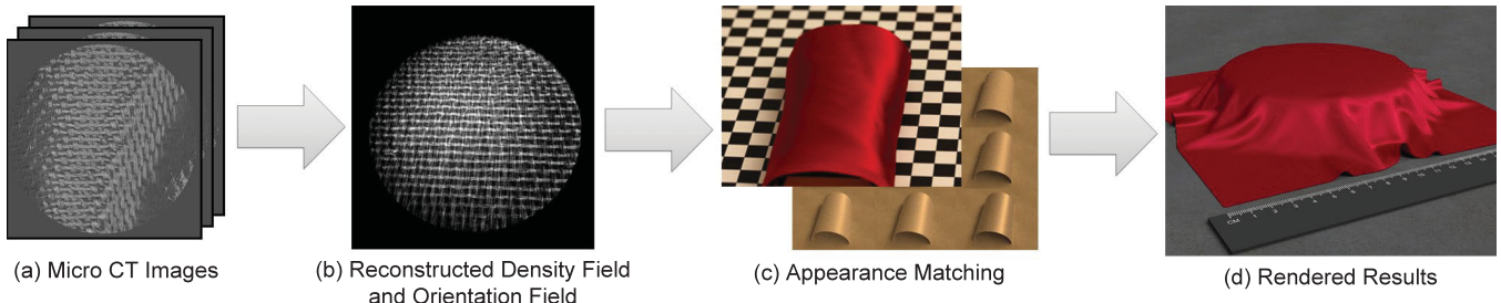
Figure 2: Our volume appearance modeling pipeline. (a) CT images are acquired, (b) the density field and orientation field of the volume are created, and (c) optical parameters of the volumetric model are assigned by matching statistics of photographs with rendered images. (d) Larger models are rendered using our acquired volumetric appearance and geometry models.
