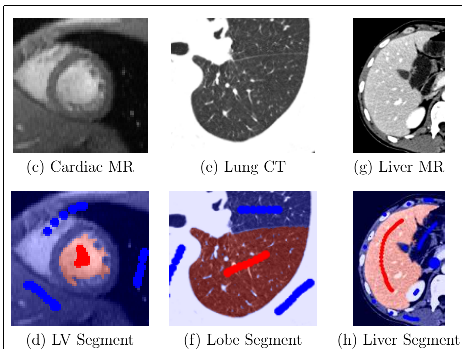
Figure 10: Segmentation Experiments
