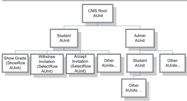
Figure 2. AUnits in CMS
