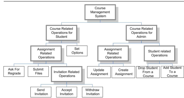
Figure 1. Course Management System
