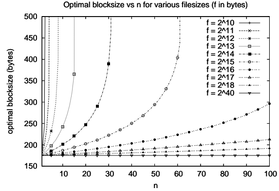
Figure 4. Optimal blocksize in bytes for a variety of file sizes f (bytes) and update intervals n using hash parameters \alpha = 0.0122348 \mu\text{sec/byte} , \beta = 1 \mu\text{sec} and s = 20 \text{ bytes} .
