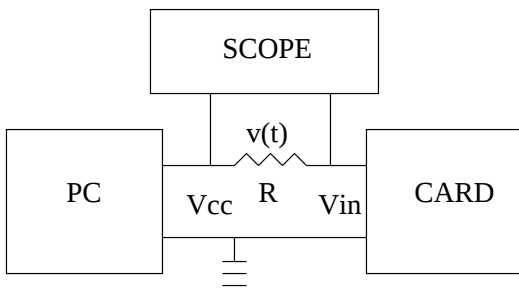
Fig. 1. Test circuit
