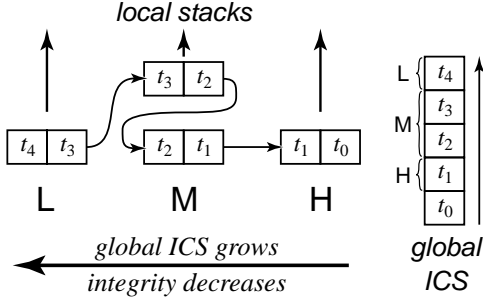
Figure 5: Distributed implementation of the global stack
