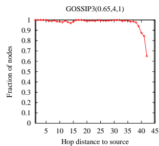
Fig. 6. \text{GOSSIP3} on a random network of degree 8.
