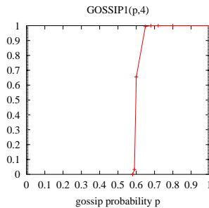
Fig. 4. \theta_4^S(p) as a function of the gossip probability p on a 1000x1000 grid.
