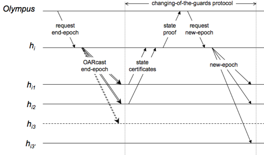
Figure 5: Example of an execution of the reconfiguration protocol. h_{i1} , h_{i2} , and h_{i3} are guards of h_i . When the Olympus suspects that h_{i3} has failed, it requests the current epoch of h_i to be concluded and installs a new set of guards, replacing h_{i3} with h_{i3'} .
