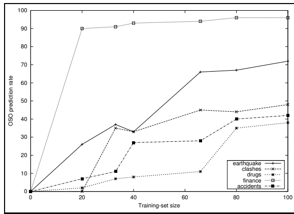
Figure 2: Ordering-task performance, in terms of OSO prediction rate, as a function of the number of documents in the training set.
