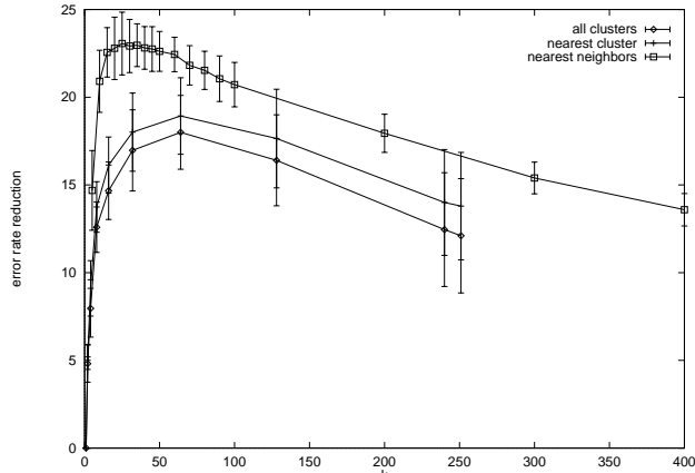
Figure 3: Average error reduction with respect to backoff on AP89 test sets.
