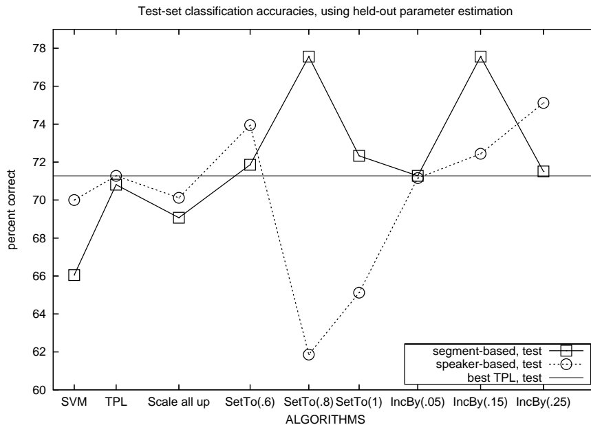
Figure 1: Experimental results. “SVM”: classification using only individual-preference information. Values of \beta are indicated in parentheses next to the relevant algorithm names.
