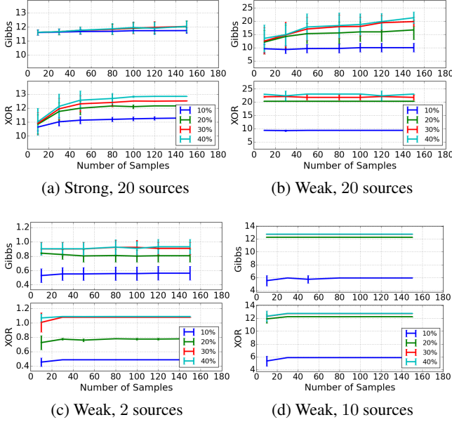
Figure 3: SAA with the XOR sampler produces better and more stable policies (e.g., larger mean and smaller error bars) than SAA with the Gibbs sampler on small networks. Y axis is the average of 10 policy values ( \times 10^3 ). Variances are illustrated by vertical bars that indicate the interval [mean - std, mean + std] (std: standard deviation). “Strong”: strong correlation. “Weak”: weak correlation. Legend: budget sizes as the percentage of the total costs of protecting all edges.
