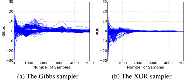
Figure 5: The effect of sample sizes on estimation of policy values. Each line corresponds to a policy. For one policy, the value of Y axis is the difference of two subsequent estimated policy values. For both the XOR and the Gibbs samplers, the difference reduces to a small value with 5,000 samples. The XOR sampler converges better and faster comparing to the Gibbs sampler.
