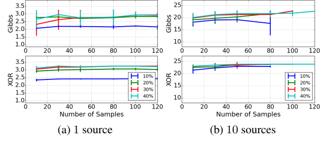
Figure 6: SAA with the XOR sampler produces better and more stable policies than SAA with the Gibbs sampler on large networks with 1 and 10 sources. Axes have the same meanings as in Fig. 3.
