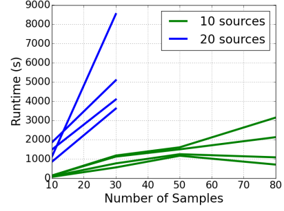
Figure 4: Runtime of MIP versus sample sizes. Lines in the same color represent different budget sizes. The runtime value is the average of 30 experiments, each with independently drawn samples.
