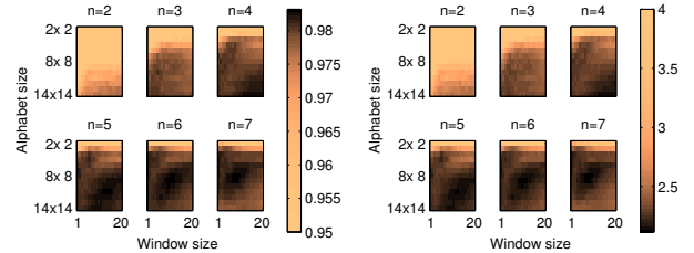
Fig. 9. cStrings correlation coefficient and RMSE values
