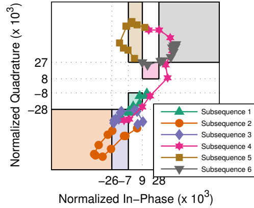
Fig. 3. 2D aggregation, SAX and n -gram construction. Every marker denotes a complex number of the time series, colored cells denote the SAX representation of the corresponding 10 complex numbers that gives rise to the alphabet letter. The alphabet size (number of equiprobable regions) in this example is 5 \times 5 and this sequence gives rise to a 6-gram. See also Figure 4 for the corresponding representation in time.
