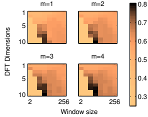
Fig. 6. DFT with power spectrum: R^2
