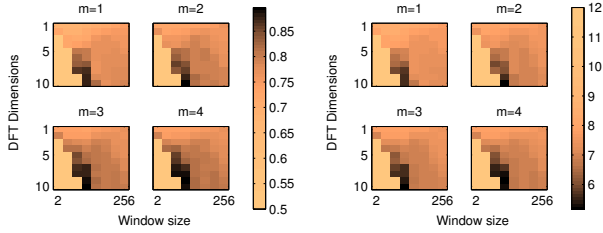
Fig. 5. DFT with power spectrum: r and RMSE
