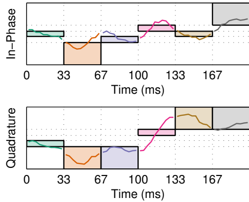
Fig. 4. Time-series representation of the in-phase and quadrature components from Figure 3
