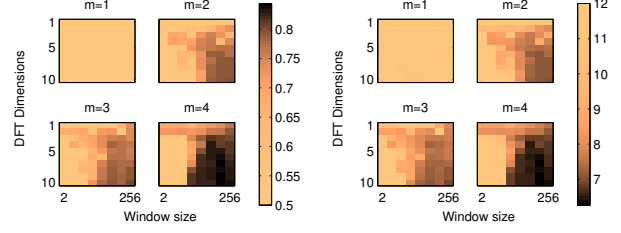
Fig. 7. DFT with complex kernel: r and RMSE
