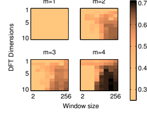
Fig. 8. DFT with complex kernel: R^2
