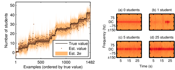
Fig. 2. (a) Predicting the number of human targets (students) in a classroom with the proposed approach based on the complex time series data from the BumbleBee sensor. (b) Typical (log) power spectrum for the radar.
