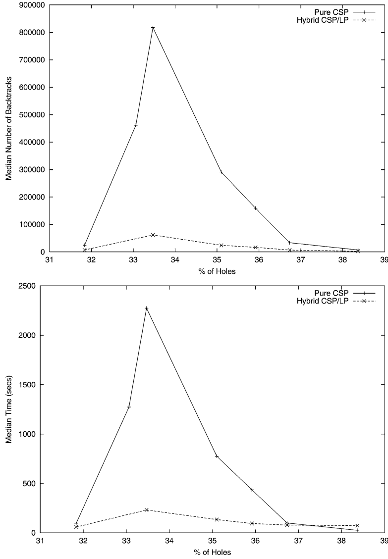
Figure 6. Median runtime (secs) for QWH instances, in the critically constrained area (order 35; 100 instances per data point).
