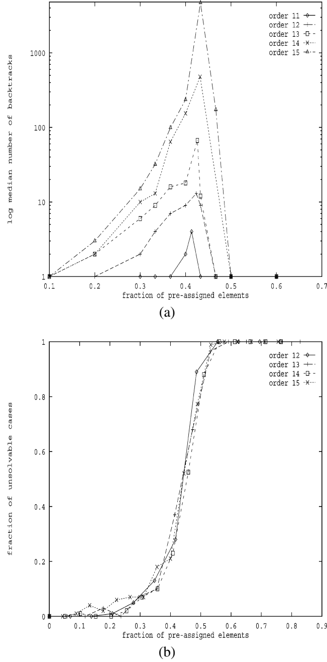
Figure 2. (a) Computational cost of solving QCP instances (order 11–15). X-axis: fraction of pre-assigned cells; Y-axis: median number of backtracks for solution (log scale). (b) Phase transition in solvability for QCP instances (order 12–15). X-axis: fraction of pre-assigned cells; Y-axis: fraction of instances for which the partial Latin square could not be completed into a full Latin square. (Each data point was computed based on 100 instances.)
