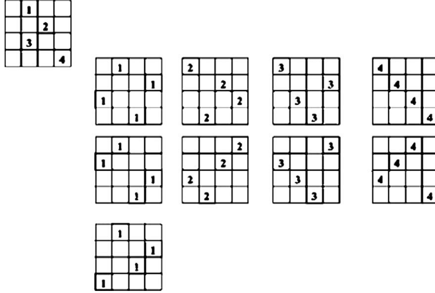
Figure 5. Families of compatible matchings for the partial Latin square in the left upper corner. For example, the family of compatible matchings for symbol 1 has three compatible matchings.
