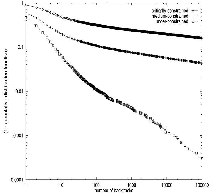
Figure 4. Heavy-tailed behavior for three different QCP instances: the top curve corresponds to a critically constrained instance; the middle curve corresponds to a medium-constrained instance; and the bottom curve corresponds to an under-constrained instance. X-axis: number of backtracks (log scale). Y-axis: the complement-to-one of the cumulative distribution (log scale) (i.e., the tail or the survival function of the distribution, \Pr\{X > x\} = 1 - F(x) , where F(x) is the cumulative distribution). The linear behavior of the curves in log-log scale indicates heavy-tailed behavior. For example, the lower curve shows that \approx 90\% of the runs finish in less than 10 backtracks; \approx 0.1\% of runs take more than 10,000 backtracks; some of the runs take even more than 100,000 backtracks. Each distribution is based on 10,000 runs of the backtrack search method. For the under-constrained instance (bottom curve) the estimate of \alpha is 0.466 \pm 0.009 . Given that \alpha < 1 and the data were obtained without censorship, the data are consistent with the hypothesis of infinite mean and infinite variance.
