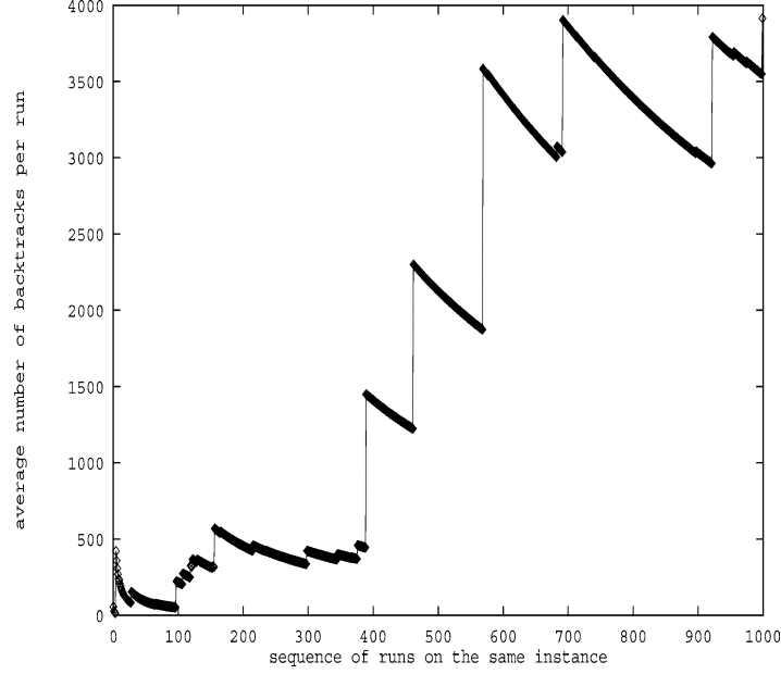
Figure 3. Erratic behavior of sample mean phenomenon. X -axis: sequence of runs on the same instance. Y -axis: average number of backtracks per run. The average of the number of backtracks until solution exhibits a very erratic behavior as we increase the number of runs of a randomized backtrack search algorithm on the same problem instance. After 200 runs, the mean is about 500 backtracks; after 600 runs, it is about 2000 backtracks; after 1000 runs, it is about 3500 backtracks. The phenomenon is due to the fact that the more runs we take into account, the more likely we hit some very long runs, which increase the overall average number of backtracks. This experiment consisted of using a randomized backtrack search algorithm (randomization only for tie breaking equal choices selected by the first-fail heuristic) on a QCP instance of order 11, with 64% of holes. Even though the randomized backtrack solver finds a solution in 50% of the cases using only one or zero backtracks (i.e., the median is 1), approximately 1% of the runs require more than 1,000,000 backtracks to find a solution.
