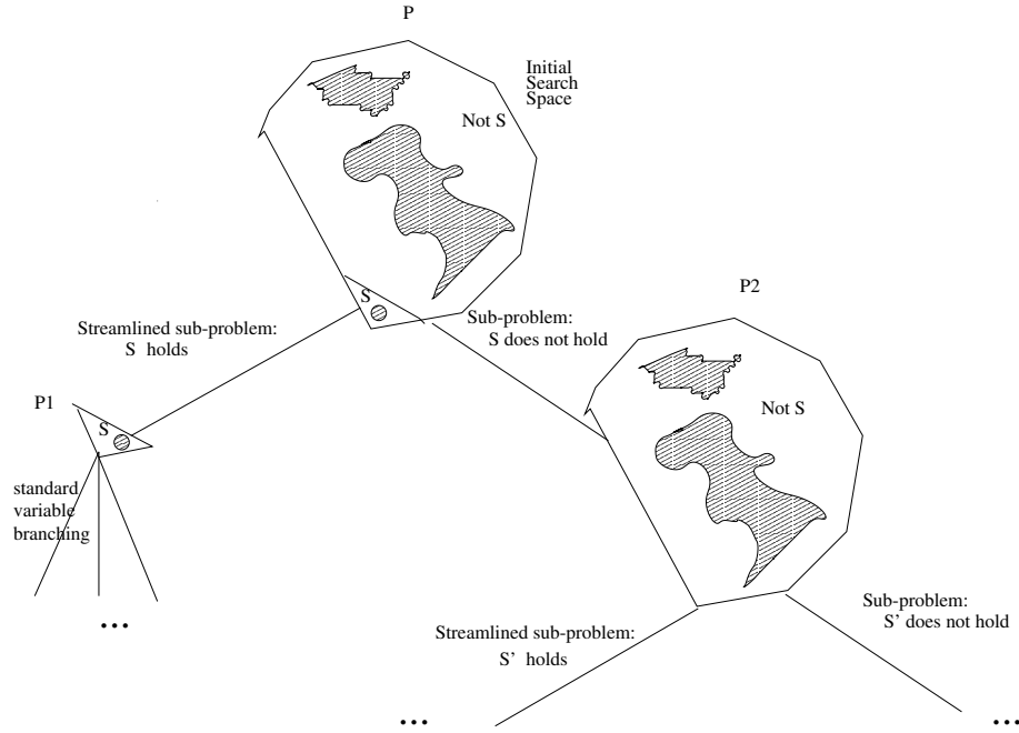
Fig. 1. Streamlining to focus the search on a small, structured part of the search space with hopefully high solution density.
