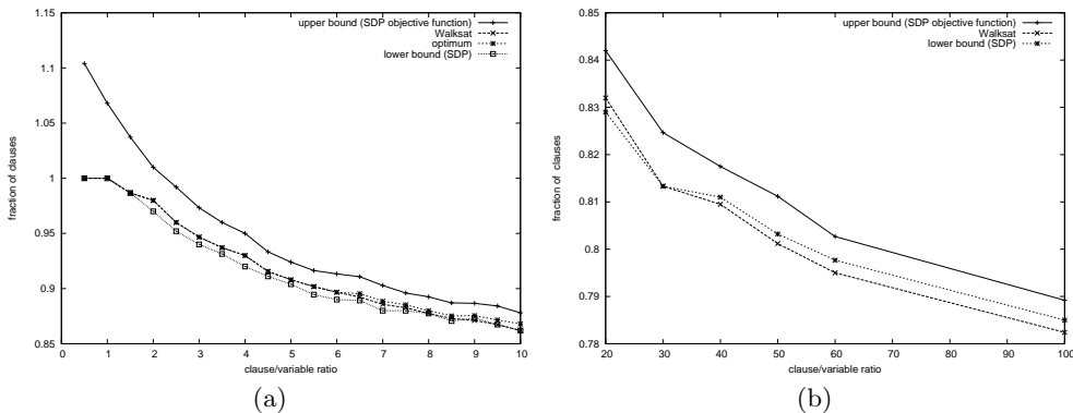
Fig. 7. SDP vs Walksat as a lower bound.
