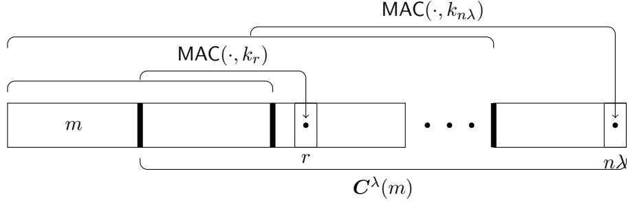
Figure 7: The structure of Known-Key Chain Signatures
