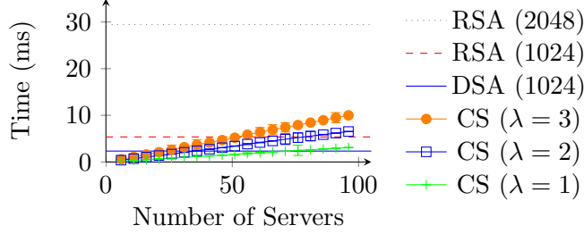
Figure 3: Execution time for generating Chain Signatures ( \epsilon = 2^{-64} )
