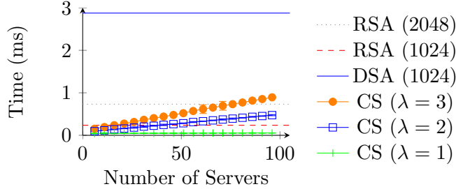
Figure 4: Execution time for checking Chain Signatures ( \epsilon = 2^{-64} )
