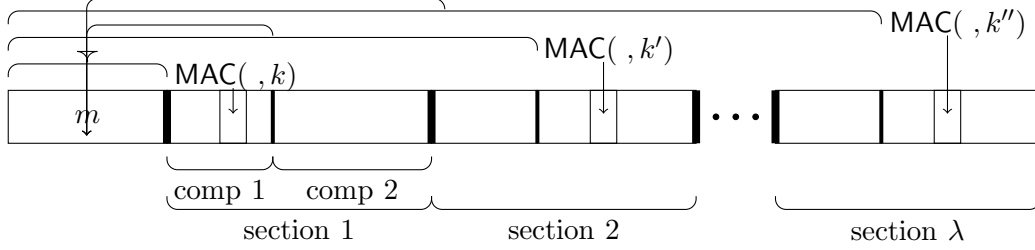
Figure 1: The structure of a signed message using Chain Signatures
