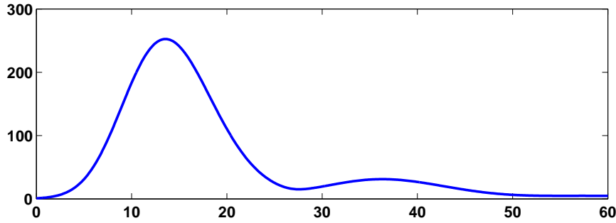
Fig. 3 \|e^{tA}\| , the hump for the transient example
