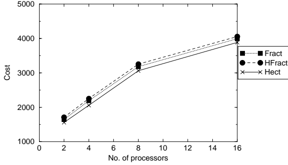
Figure 9: Costs for Uniform Distribution without load
