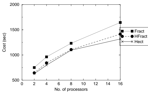
Figure 12: Costs for Uniform Distribution with load (migration)
