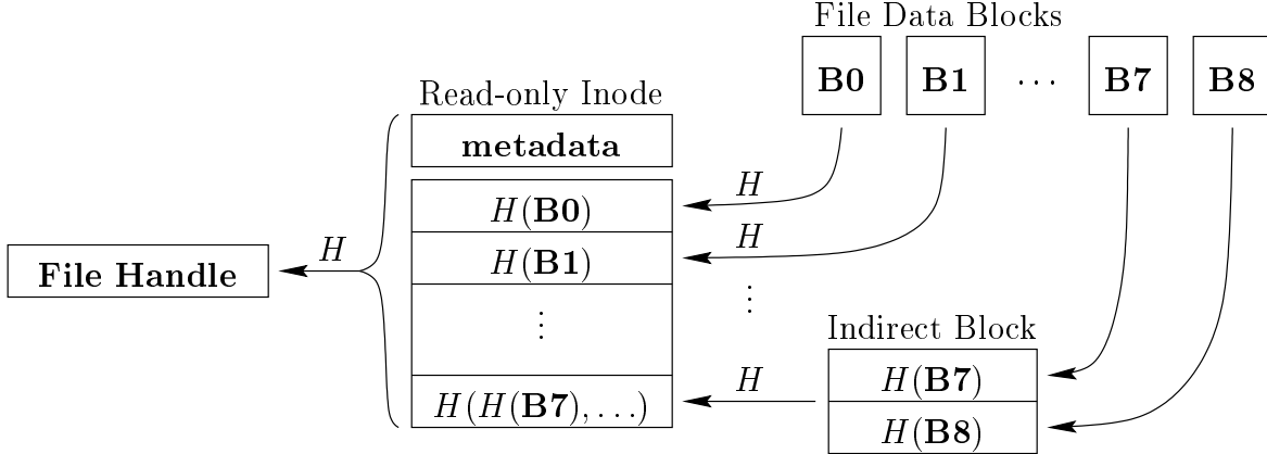
Figure 4: Format of a read-only file system inode.
