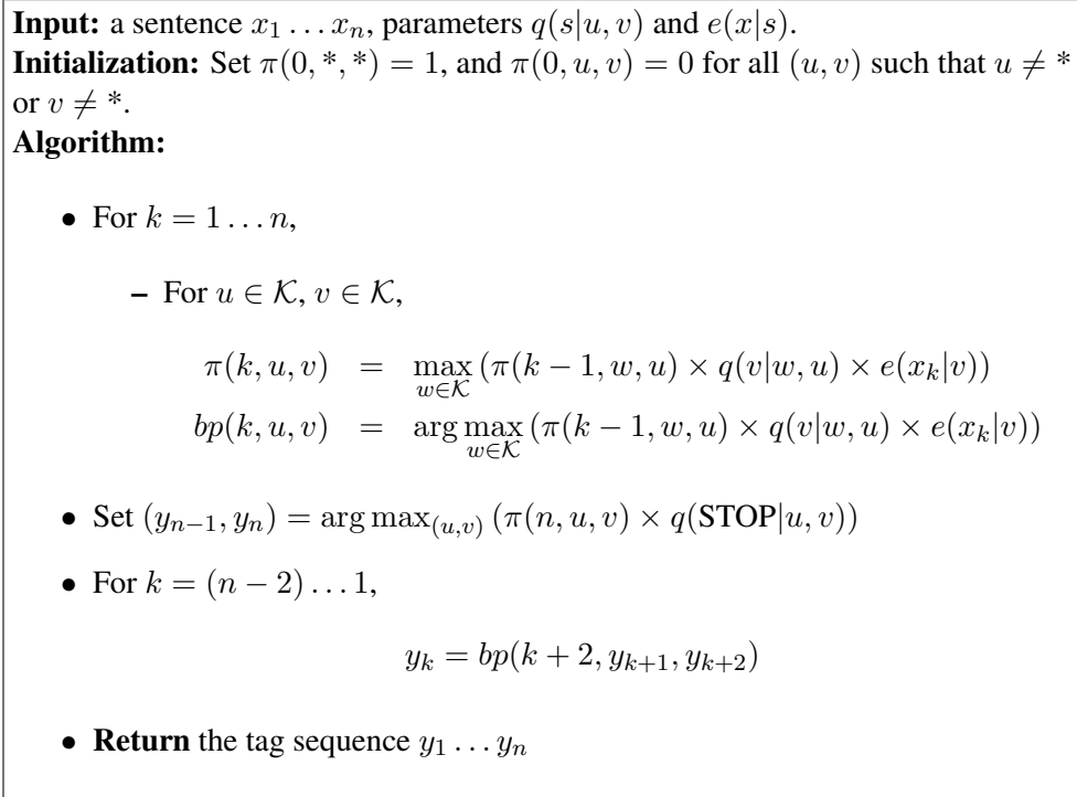
Figure 2: The Viterbi Algorithm with backpointers.
