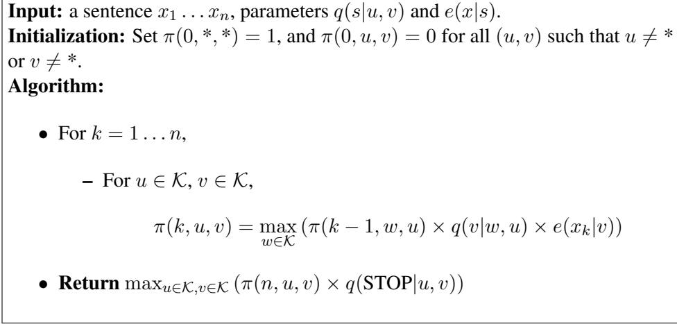
Figure 1: The basic Viterbi Algorithm.
