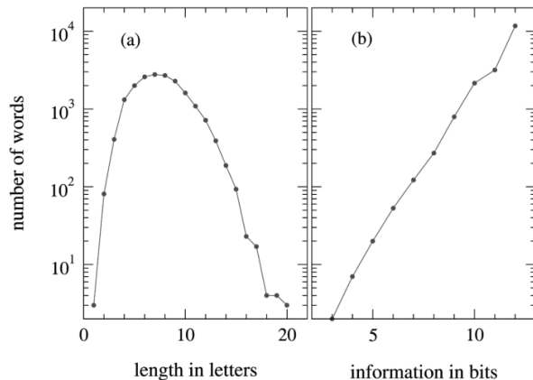
Figure 7. (a) Histogram of the lengths in letters of all distinct words in the text of the novel Moby Dick . (b) Histogram of the information content a la Shannon of words in Moby Dick . The former does not, by any stretch of the imagination, follow an exponential, but the latter could easily be said to do so. (Note that the vertical axes are logarithmic.)
