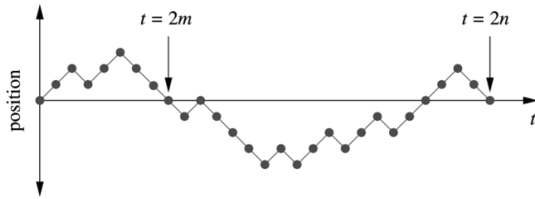
Figure 9. The position of a one-dimensional random walker (vertical axis) as a function of time (horizontal axis). The probability u_{2n} that the walk returns to zero at time t = 2n is equal to the probability f_{2m} that it returns to zero for the first time at some earlier time t = 2m , multiplied by the probability u_{2n-2m} that it returns again a time 2n-2m later, summed over all possible values of m . We can use this observation to write a consistency relation, equation (52), which can be solved for f_t , equation (60).
