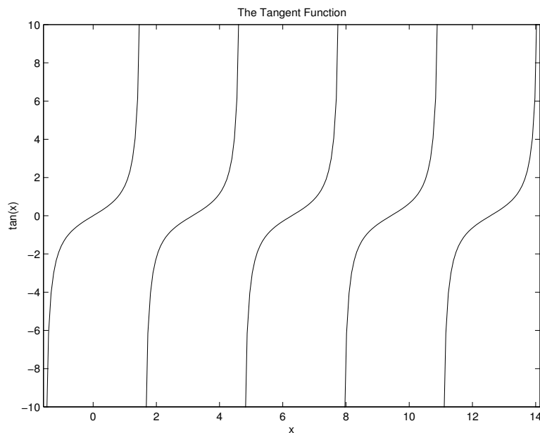
FIGURE 1.5 A plot of \tan(x)
