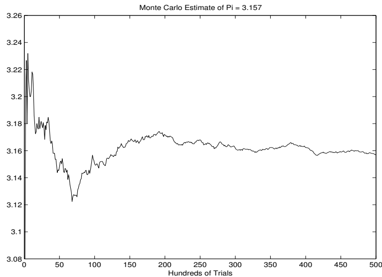
FIGURE 1.11 A Monte Carlo estimate of \pi
