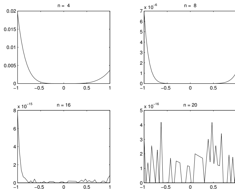
FIGURE 1.17 Relative error in T_n(x)
