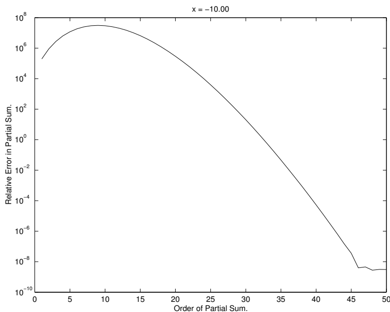
FIGURE 1.15 Error in Taylor approximations to e^x , x = -10
