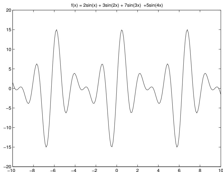
FIGURE 1.8 A sum of sines
