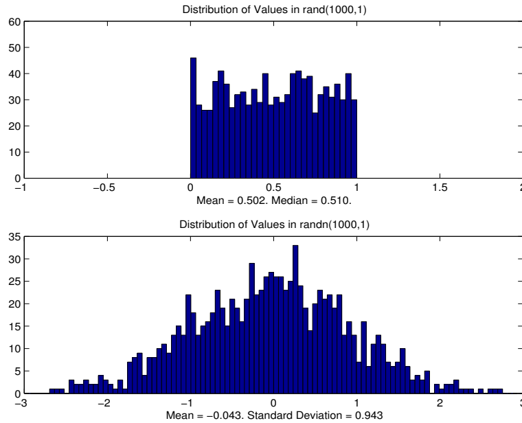
FIGURE 1.9 The uniform and normal distributions
