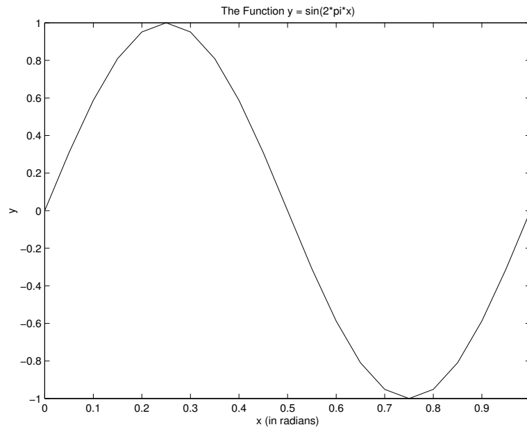
FIGURE 1.1 A crude plot of \sin(2\pi x)
