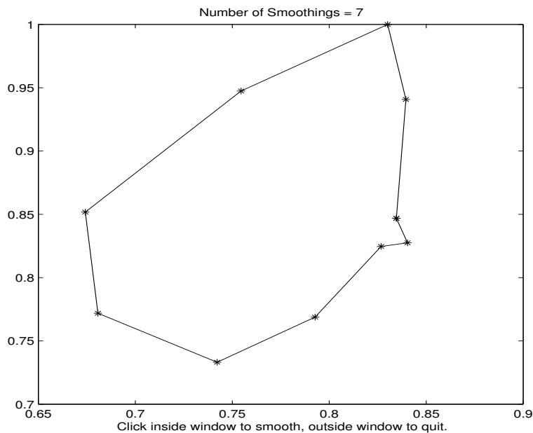
FIGURE 1.13 A smoothed polygon
