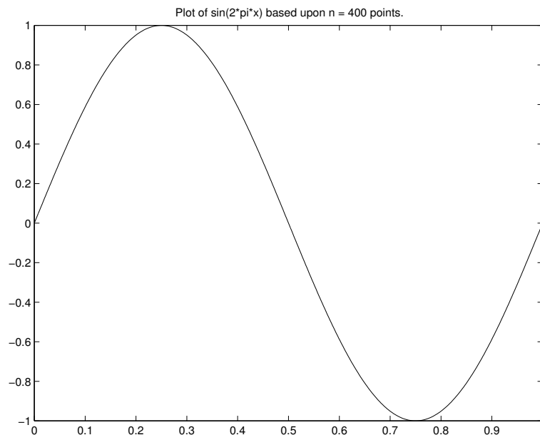
FIGURE 1.4 A smooth plot of \sin(2\pi x)
