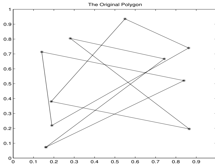
FIGURE 1.12 The initial polygon
