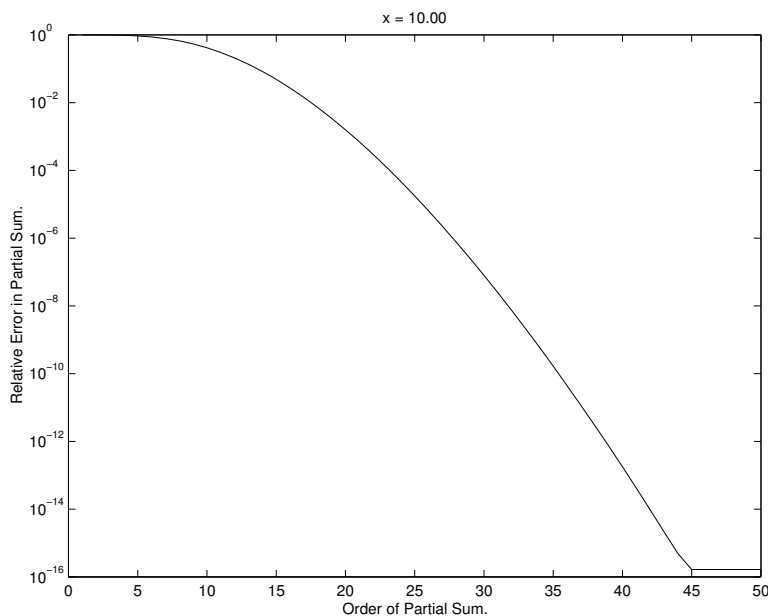
FIGURE 1.14 Error in Taylor approximations to e^x , x = 10
