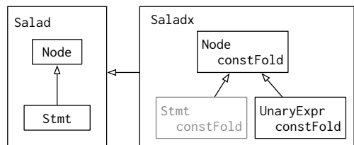
Figure 1. Applying family polymorphism to compiler construction.
