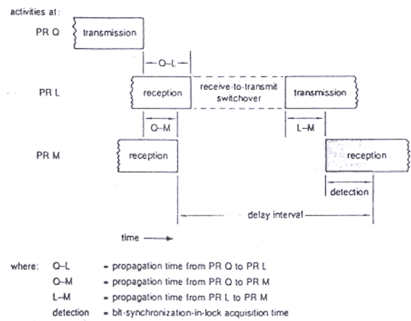
Fig. 9. CSMA delay interval.
