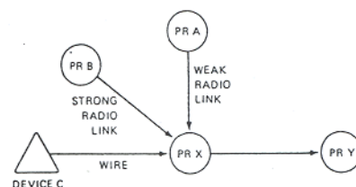
Fig. 8. LPR with variable-strength receive links.
