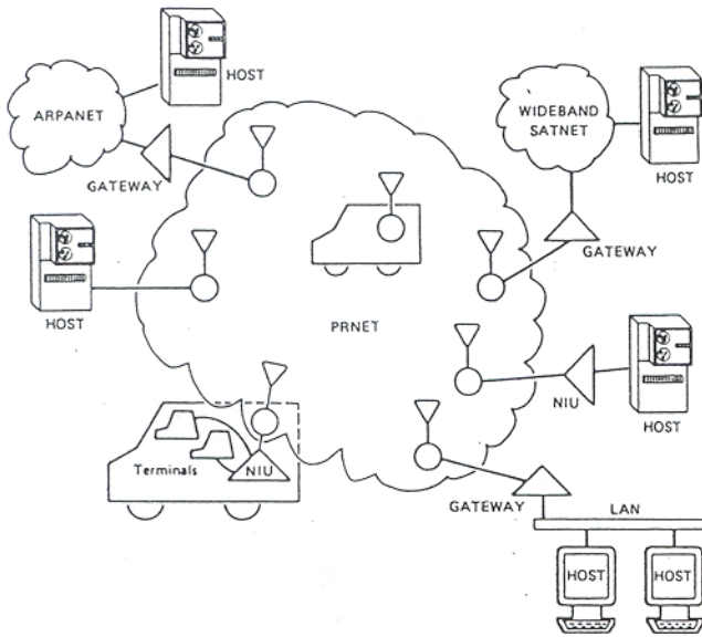
Fig. 4. Packet radio network in the Internet.
