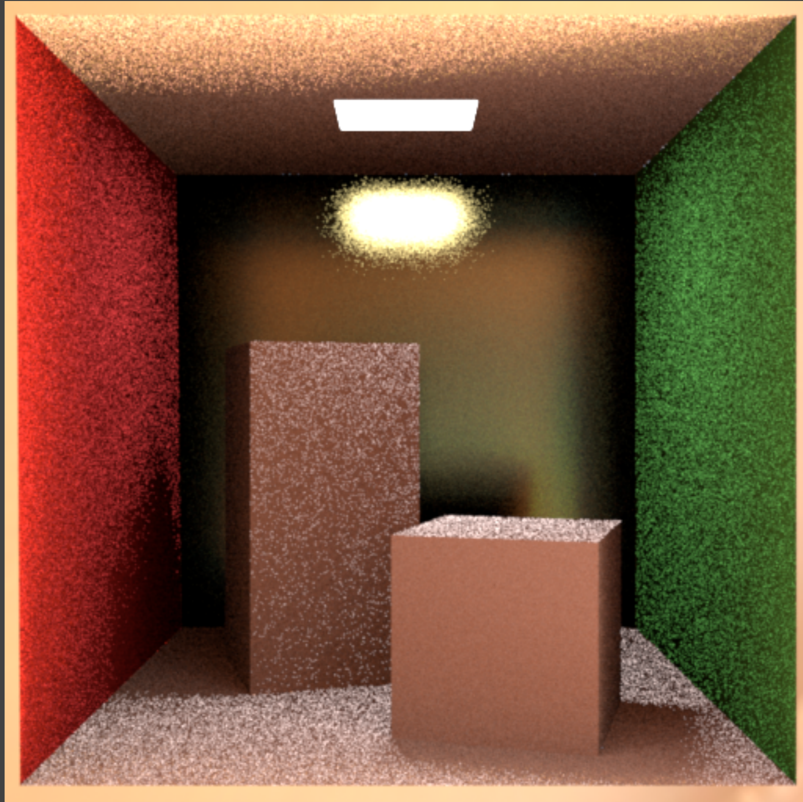
sampling the BRDF
