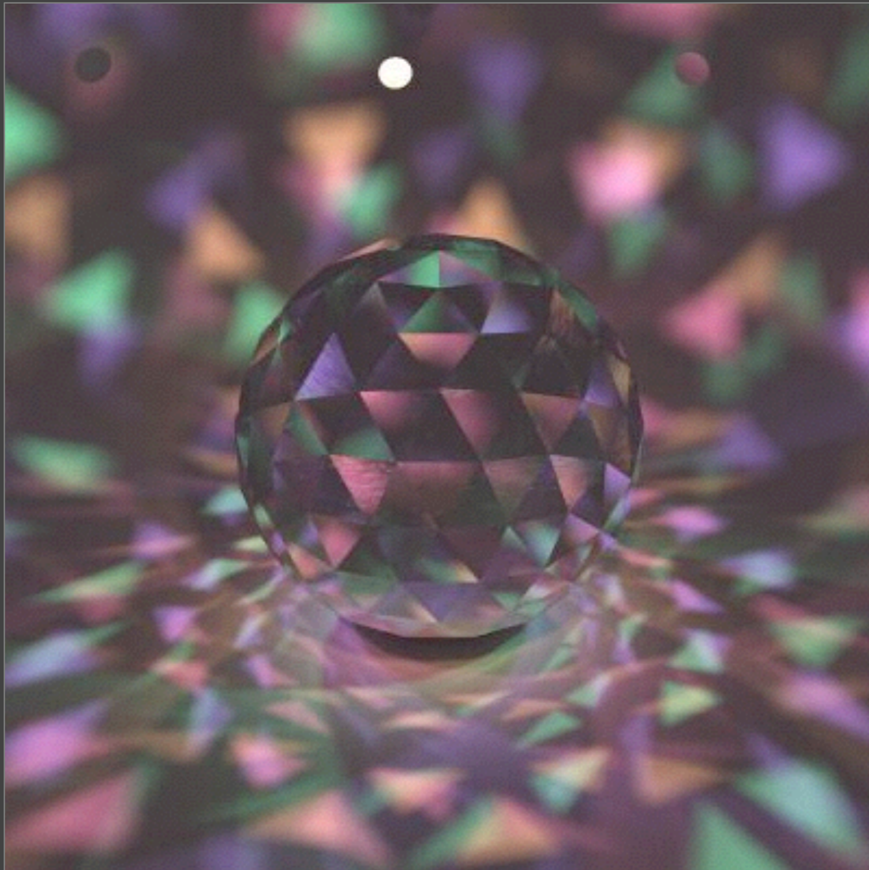
Kelemen et al. 2002 Primary sample space MCMC
